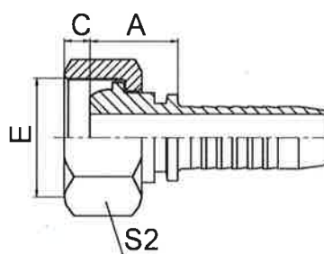
SW20111-T METRIC FEMALE MULTISEAL
