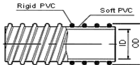
"Cross-sectional View"
